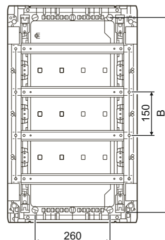
Fixing centre distances and distance between rails
