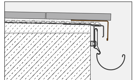
Schlüter®-DITRA-DRAIN-STU
