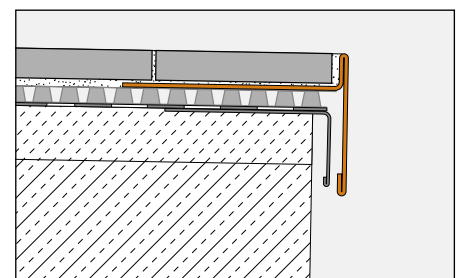
Schlüter®-DITRA-DRAIN-STU
